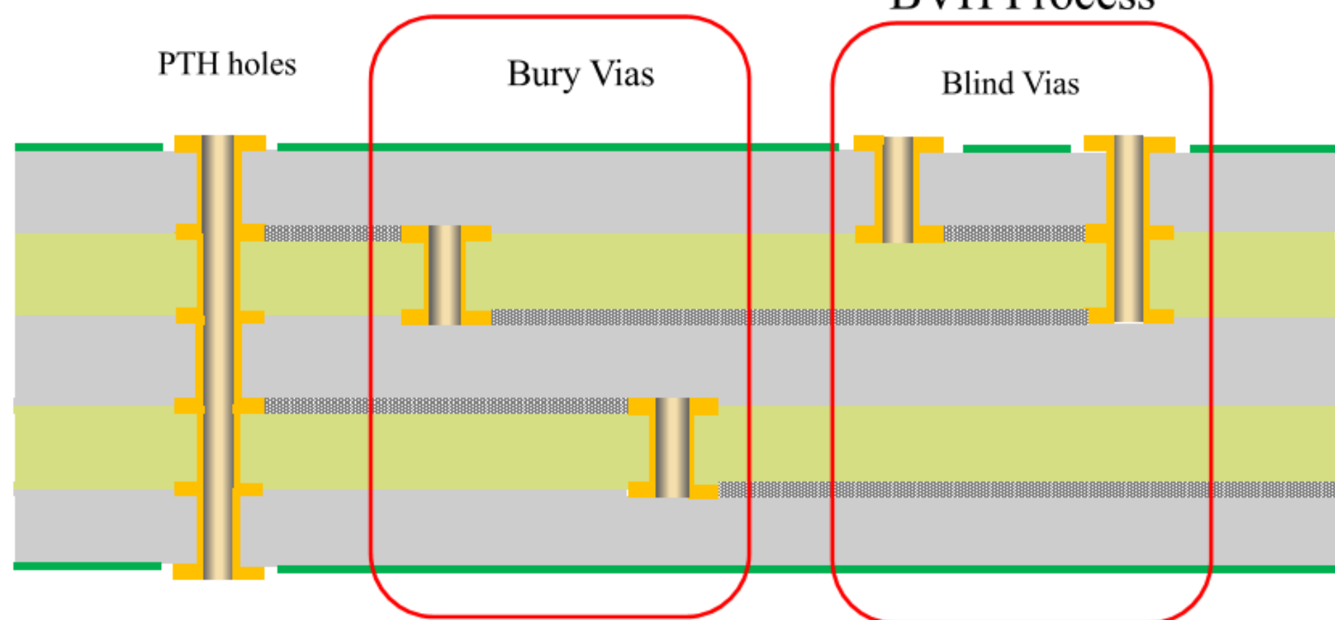
BVH Process
